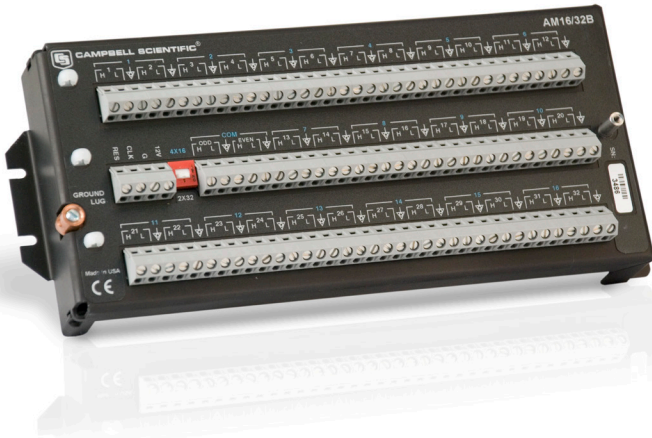
The CR1000 is compatible with the AM16/32B (shown above) and AM25T multiplexers.
